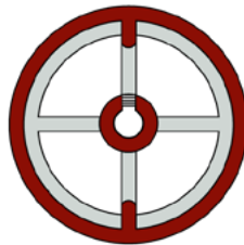
Bored Hole With Setscrew Hole Over Keyway
